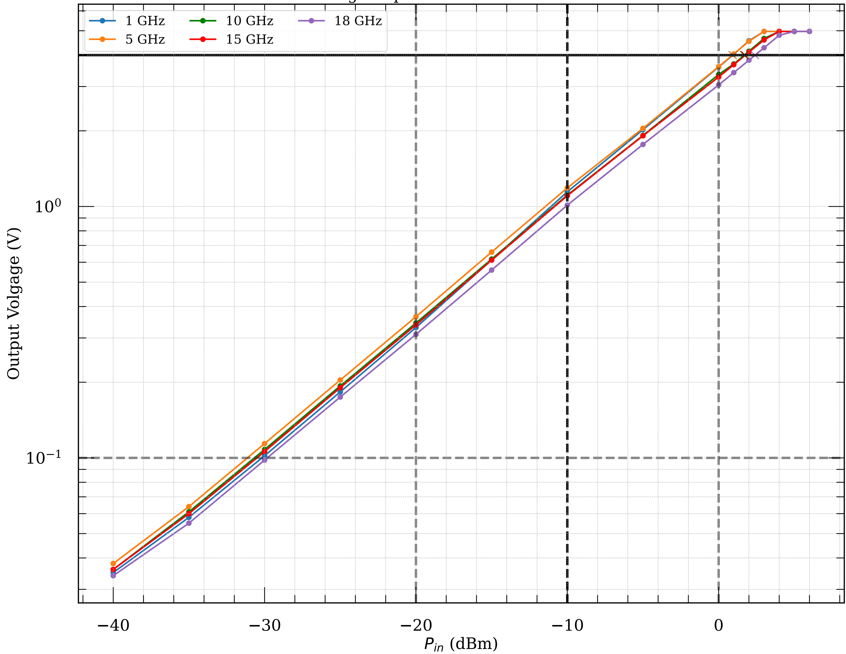
Measured voltage-to-power curve of detector module064v2
